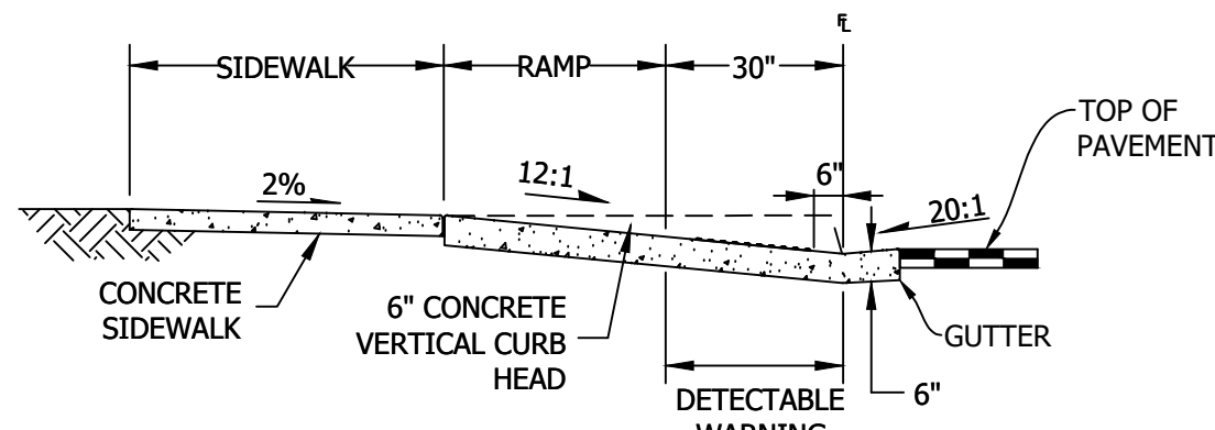
TYPICAL CURB RAMP SECTION A-A
