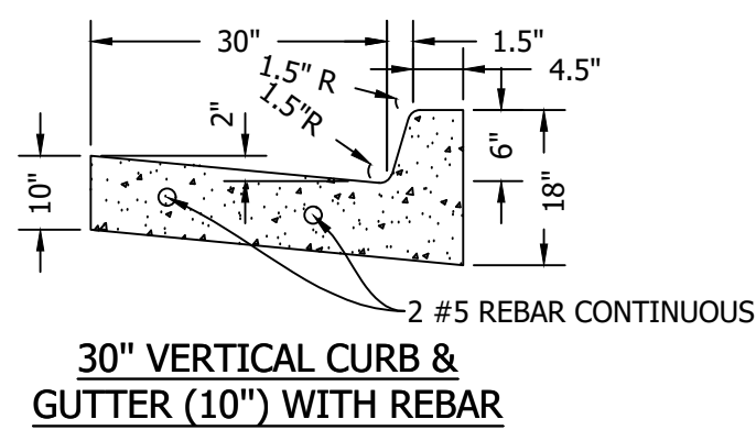
30" VERTICAL CURB & GUTTER (10") WITH REBAR
