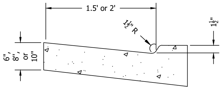
TYPICAL CURB & GUTTER AT DRIVEWAY
