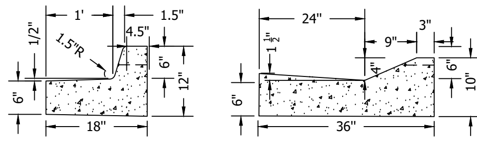
18" MEDIAN CURB & GUTTER
