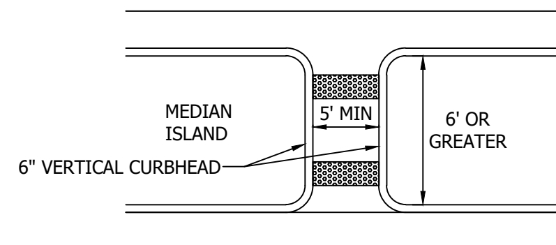
TYPE 2 MEDIAN ISLAND RAMP PLAN
