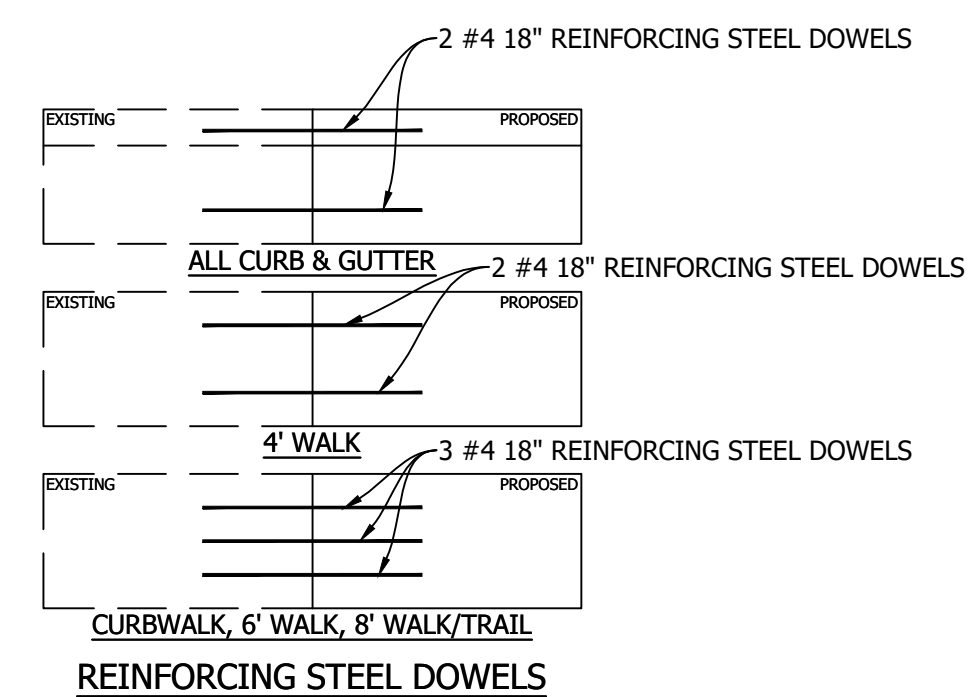
REINFORCING STEEL DOWELS
