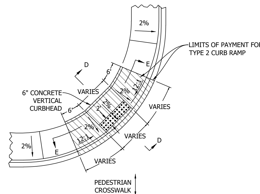
TYPE 2 TYPICAL CURB RAMP PLAN
