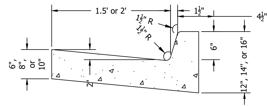
VERTICAL CURB & GUTTER
