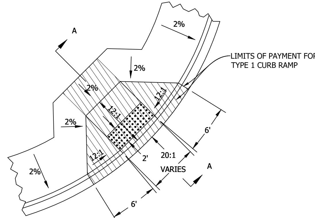
TYPE 1 TYPICAL CURB RAMP PLAN
