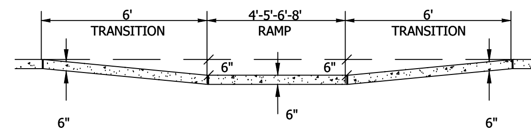
TYPE 2 TYPICAL CURB RAMP SECTION E-E
