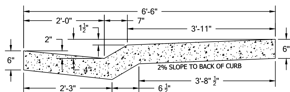
6'- 6" X 6" CURBWALK
