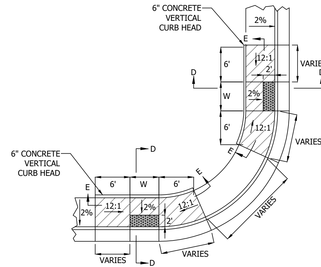
TYPE 2 BI-DIRECTIONAL TYPICAL CURB RAMP PLAN
