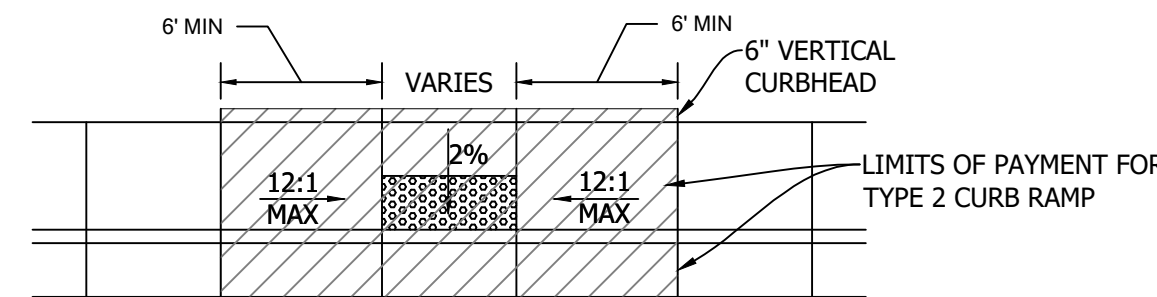
TYPE 2 MIDBLOCK RAMP PLAN
