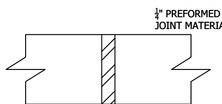
EXPANSION JOINT
