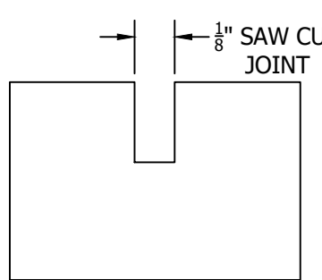
SAW CUT JOINT DEPTH OF JOINT SHALL BE 1" DEEP IN 6" THICK CONCRETE
