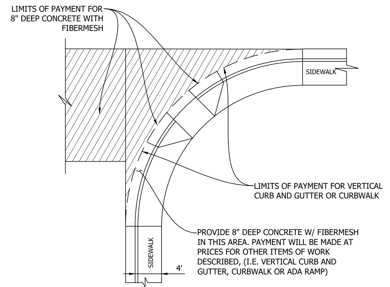
PAVEMENT LIMITS AT SQUARED RADIUS RETURN
