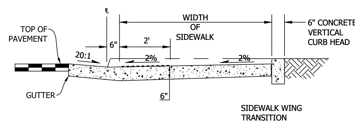
TYPE 2 TYPICAL CURB RAMP SECTION D-D
