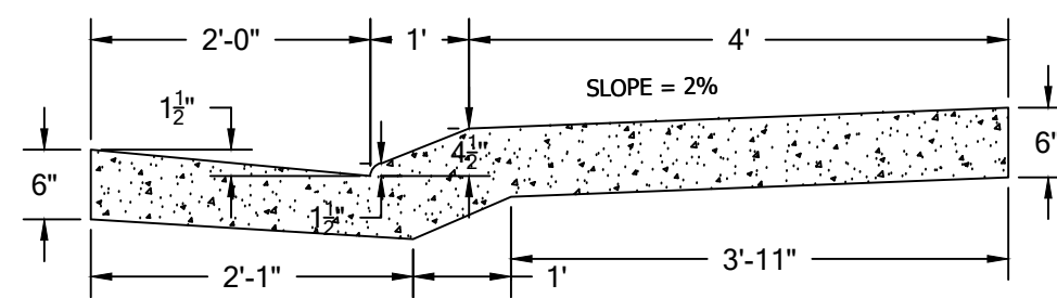
7'- 0" X 6" CURBWALK
