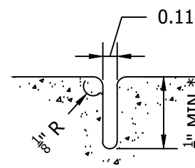
CONTRACTION OR WEAKENED PLANE JOINT
