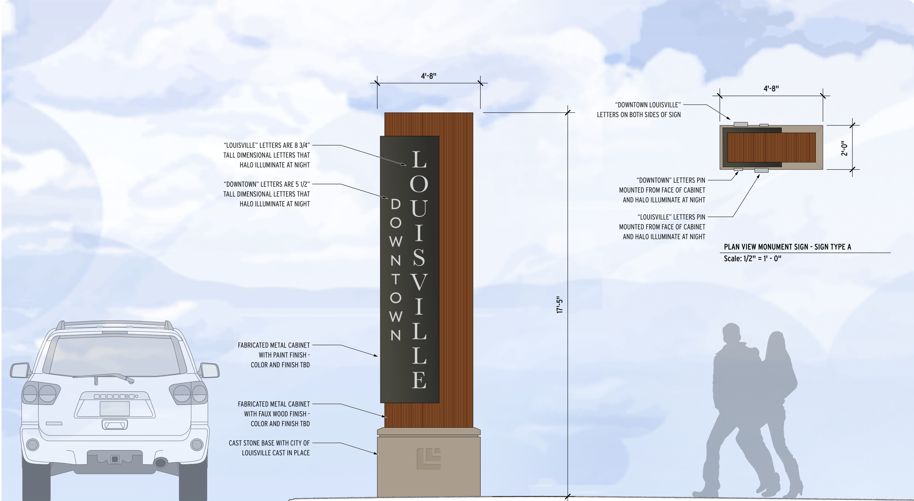
DOWNTOWN LOUISVILLE MONUMENT SIGN - SIGN TYPE A Scale: 1/2" = 1' - 0"
