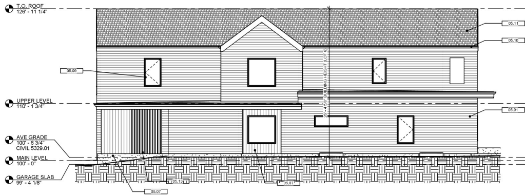
② SDP - EAST ELEVATION (REFERENCE LOT 4) 3/16" = 1'-0"
