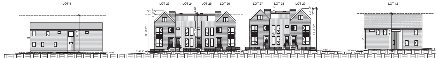
SITE - LOTS 23-29 WEST ELEVATION ④ HEIGHT EXHIBIT 1/16" = 1'-0"
