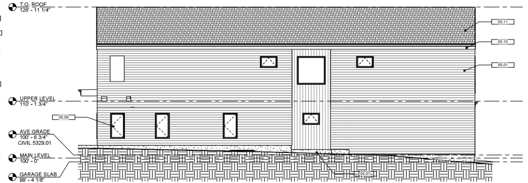
③ SDP - WEST ELEVATION (REFERENCE LOT 4) 3/16" = 1'-0"
