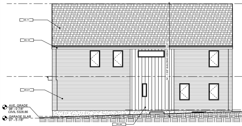
② SDP - WEST ELEVATION 3/16" = 1'-0"
