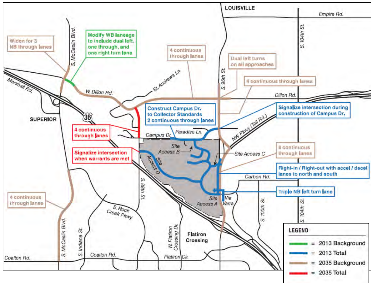
Figure B.1 Summary of Roadway Improvements (ConocoPhillips Campus TIS)
