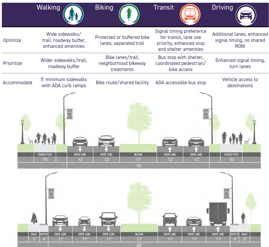
Figure 5. Great/Complete Street Graphic from the City of Louisville's TMP
