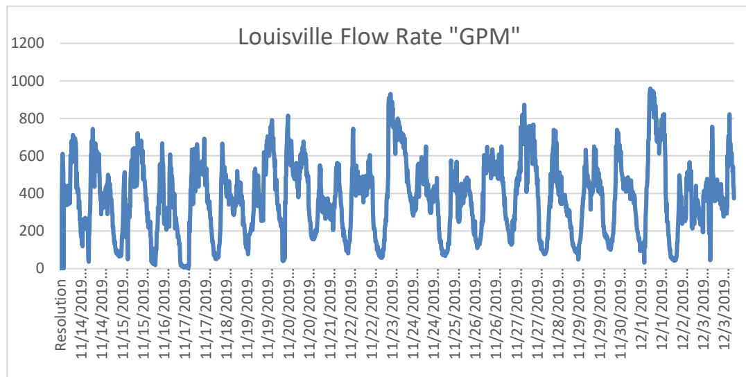
Figure 1: Connection Point Flow Monitoring
