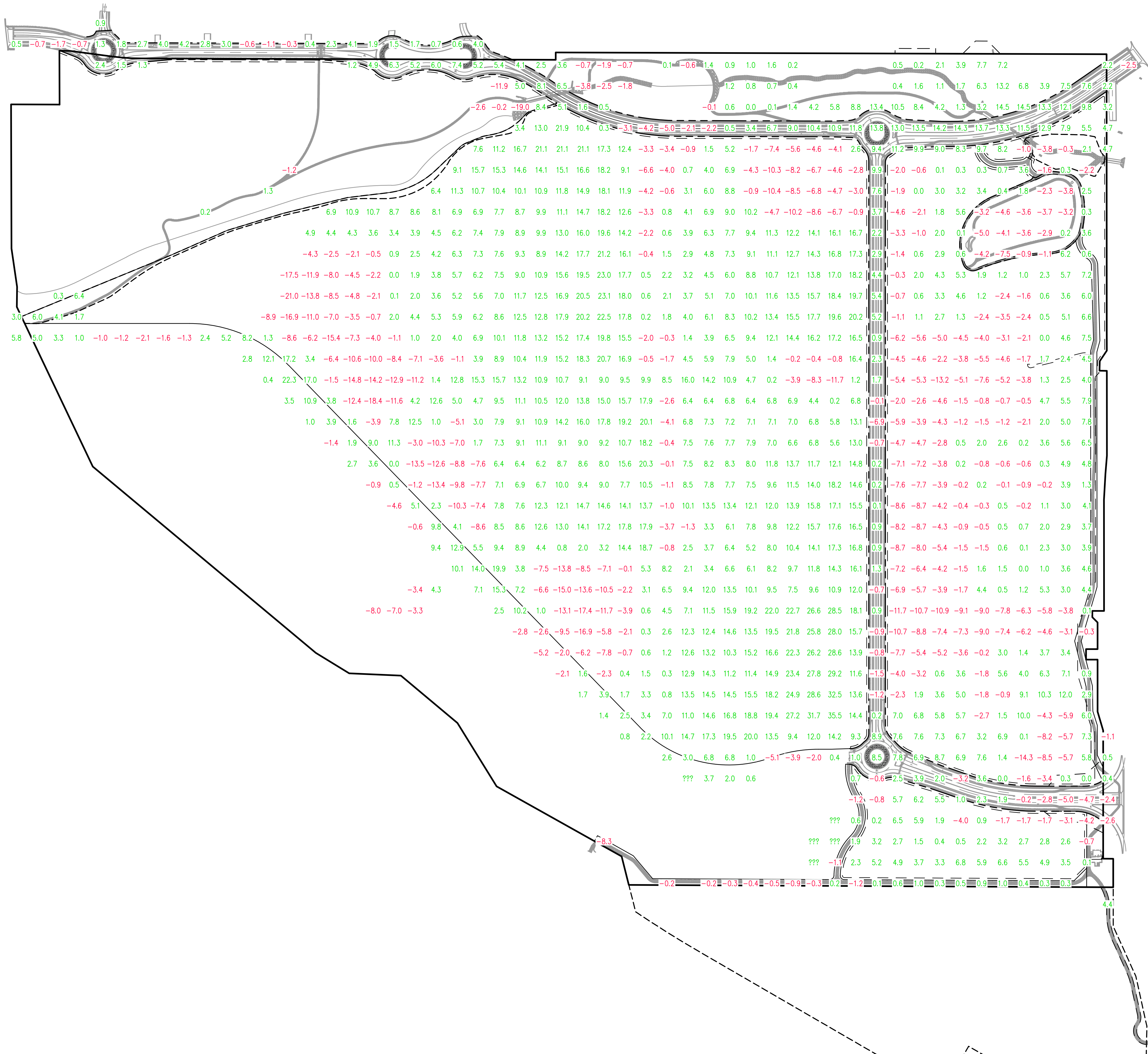
REDTAIL RIDGE TOTAL SITE - CUT & FILL MAP
